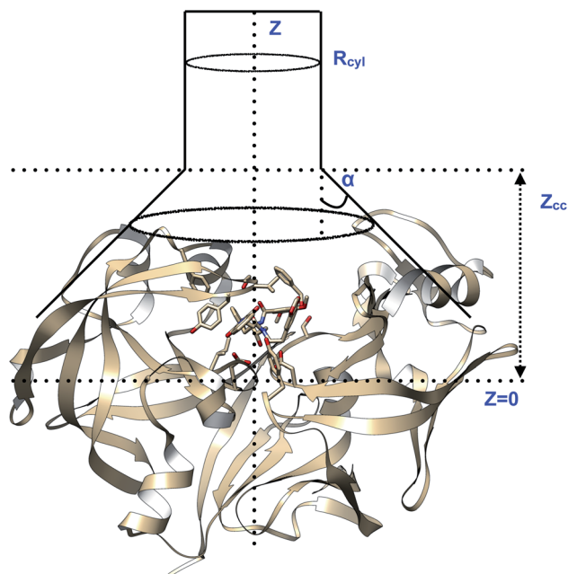
Fig. 23 Pictorial representation of a model funnel shaped potential that can be used to calculate binding free energy and binding/unbinding induced conformational changes in PAPs. R_{cyl} describes the radius of the cylindrical section and Z defines the axis to study binding/unbinding. Z can be COM_{unbind} or some other distance based order parameter. Z_{cc} is the distance where the potential switches from cone to cylindrical shape. The effect of restraint potential can be rigorously calculated as described in ref. 92. R_{cyl} should be adjusted such that it doesn't affect the natural conformational dynamics of the ligand binding/unbinding. PAP-inhibitor complex provides a true challenge (compared to T4-lysozyme and other systems where the ligand has few torsional degrees of freedom and protein is relatively rigid ) for funnel metadynamics as the ligands have large number of torsion angles and the protein undergoes large conformational changes during binding/unbinding. Abstract order parameters e.g. TICA/SGOOP/VAC, path CVs can address this challenge. Funnel metadynamics using open flap inhibitors can in principle give insights into how flipping of Tyr and Trp accommodate bigger ligands which has direct application in ligand design.
