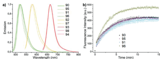
Fig. 16 (a) Normalized emission spectra of compounds 90–98 . (b) Time course of fluorogenic DA_{inv} between green emitting tetrazine dyes and TCO (500 nM in PBS each). Reproduced with permission of ref. 58. Published by The Royal Society of Chemistry.
