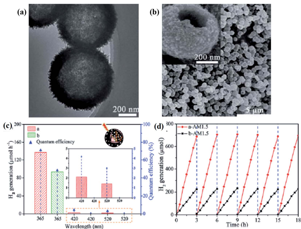
Fig. 24 (a) TEM image and (b) SEM image of the stable mesoporous B-TiO 2 hollow spheres, (c) photocatalytic hydrogen production rate by the mesoporous hollow spheres, and (d) cycling check for the stability of the mesoporous B-TiO 2 hollow sphere. Reprinted with permission from ref. 110. Copyright 2013, Royal Society of Chemistry.
