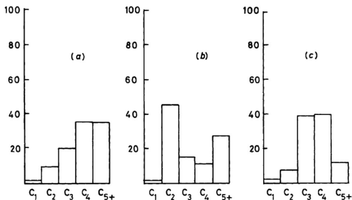
Fig. 7 Comparison of the product selectivities for the reaction of methanol and methylating agents over H-ZSM-5 at 250 °C. (a) \text{CH}_3\text{OH} (WHSV 0.005 \text{h}^{-1} , 87% conversion), (b) (\text{CH}_3)_2\text{SO}_4 (WHSV 0.075 \text{h}^{-1} , conversion 21%), (c) \text{CH}_3\text{I} (WHSV 0.06 \text{h}^{-1} , conversion 0.1%). Reproduced with permission from ref. 25.
