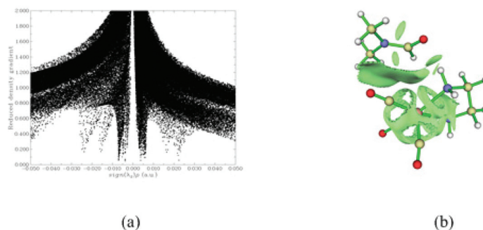
Scheme 2 Scatter graphs of the RDG vs. \text{sign}(\lambda_2)\rho(r) correlations (a) along with the 3D RDG isosurfaces (isosurface = 0.70 au) for the \text{ImA1}\cdots\text{DMF} intermediate calculated at the \text{wB97XD/Def2-TZVP} level of theory.
