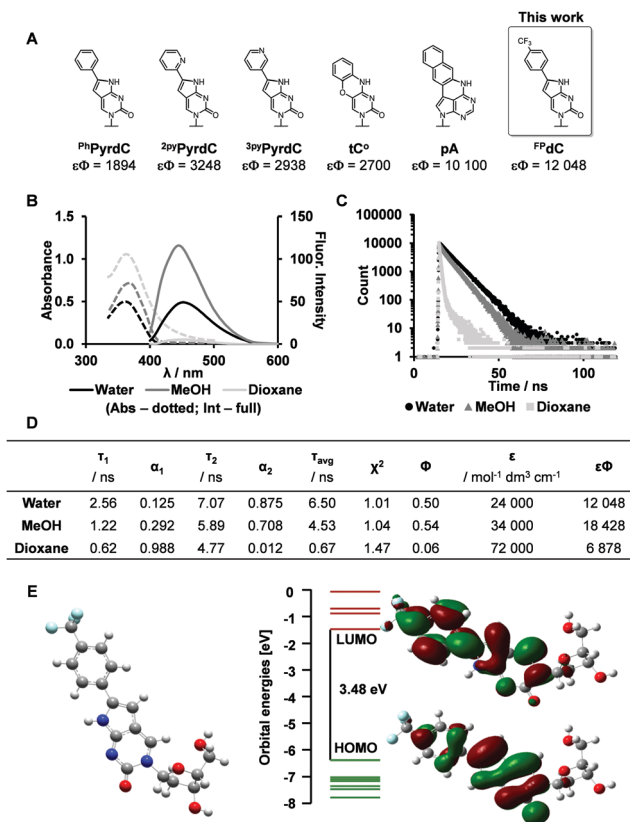
Fig. 1 Synthesis and photophysical properties of FPdC. (A) Reported cytidine analogues and their brightness ( \epsilon\Phi ) in buffer. 29–31 (B and C) Absorbance and emission spectra, as well as fluorescence decay of FPdC (dotted lines: Absorbance, full lines: Fluorescence). (D) Quantified photophysical properties of FPdC. (E) DFT minimized geometry of FPdC and its HOMO and LUMO orbitals.
