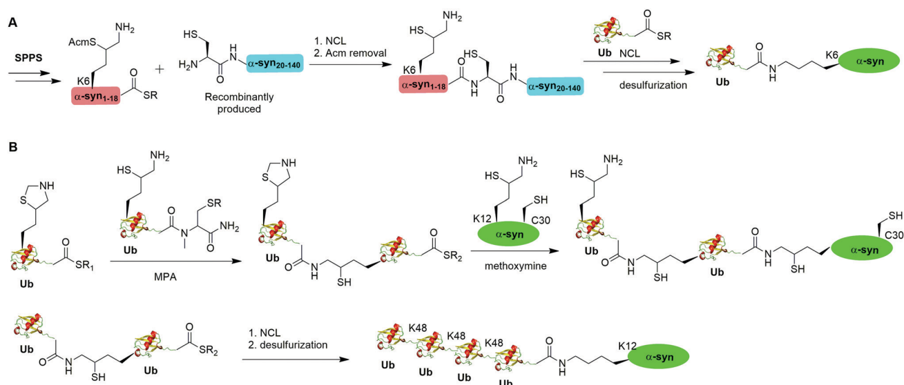
Fig. 6 \delta -Mercaptolysine-mediated NCL to generate mono- and ploy-ubiquitinated \alpha -syn. (A) \delta -Mercaptolysine-mediated NCL to generate mono-ubiquitinated \alpha -syn. (B) \delta -Mercaptolysine-mediated NCL to generate ploy-ubiquitinated \alpha -syn.
