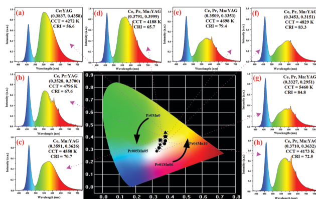
Fig. 6 Electroluminescence spectra and chromaticity parameters of the corresponding white LEDs driven by a 350 mA current: (a) Pr0Mn0, (b) Pr02Mn0, (c) Pr0Mn04, (d–h) Pr005Mn05, Pr01Mn06, Pr015Mn07, Pr02Mn08, Pr04Mn10.
