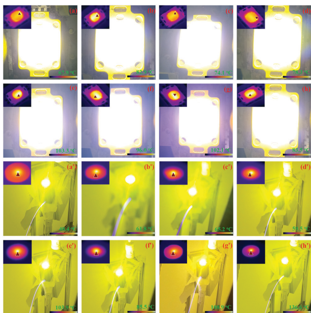
Fig. 5 Photographs of the lighting of white LEDs/LDs devices and corresponding infrared thermal images of (a/a') Pr0Mn0, (b/b') Pr02Mn0, (c/c') Pr0Mn04, (d/d') Pr005Mn05, (e/e') Pr01Mn06, (f/f') Pr015Mn07, (g/g') Pr02Mn08, and (h/h') Pr04Mn10 excited by blue LEDs/LDs.
