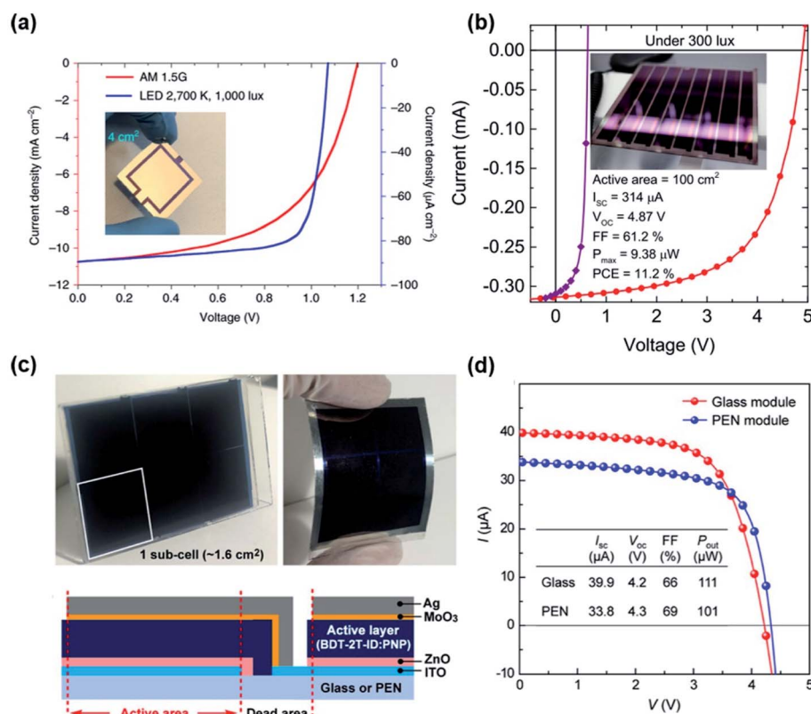
Fig. 2 (a) J-V characteristics of an OPV device with a 4.0 \text{ cm}^2 -large area under 1 sun and an LED illumination. Inset: a photograph of the 4 \text{ cm}^2 device. Reproduced with ref. 17 with permission from Springer Nature. (b) J-V characteristics of an 8-pixel module OPV device (red) with a total active area of 100 \text{ cm}^2 and a pixel (purple), respectively under FL at 300 lx. Inset: a photograph taken of this module. Reproduced with ref. 23 with permission from AIP Publishing. (c) Photographs, schematic and (d) J-V characteristics of 6 series-connected devices fabricated on a glass substrate and a flexible substrate. Reproduced with ref. 38 with permission from the American Chemical Society.
