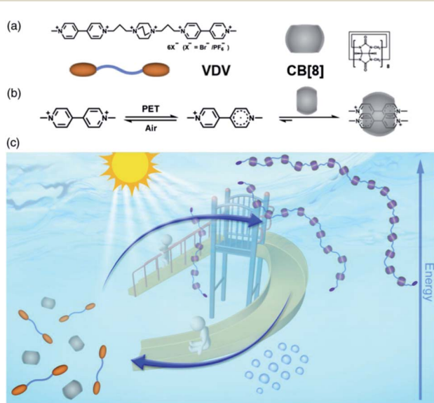
Fig. 18 Light powered dissipative supramolecular polymerization system based on a MV •+ dimer stabilized in cucurbit[8]uril. Reproduced from ref. 85 with permission from Chinese Chemical Society, Copyright 2019.
