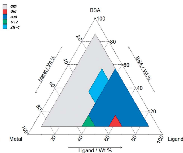
Fig. 1 Ternary diagrams (by weight fraction, see Table S1† for details) of BSA, HmIM (labelled as ligand) and \text{Zn}(\text{OAc})_2 \cdot 2\text{H}_2\text{O} (labelled as metal). TD-H 2 O (a) represents the main phases (>50 wt, see Table S2† for details) obtained by washing the sample with DI water. TD-EtOH (b) represents the main phases (>50 wt, see Table S3† for details) obtained by washing the sample first with DI water and then with ethanol. The total mass of the reagent was chosen by selecting a value in between those previously reported in the literature (see ESI† for further details). 11,34
