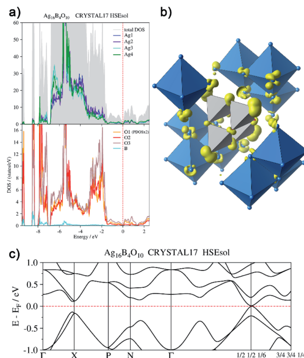
Fig. 7 (a) Total and atom-projected density of states, (b) isosurface ( 0.04 \text{ e}^- \text{ \AA}^{-3} ) of the electron density generated by the bands below the Fermi level ( E_F = -1.44 \text{ eV} to E_F ), (c) bands at E_F .
