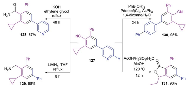
Scheme 36 NHC-catalyzed [4 + 2] benzannulation to synthesize cyano-bearing functional benzenes.
