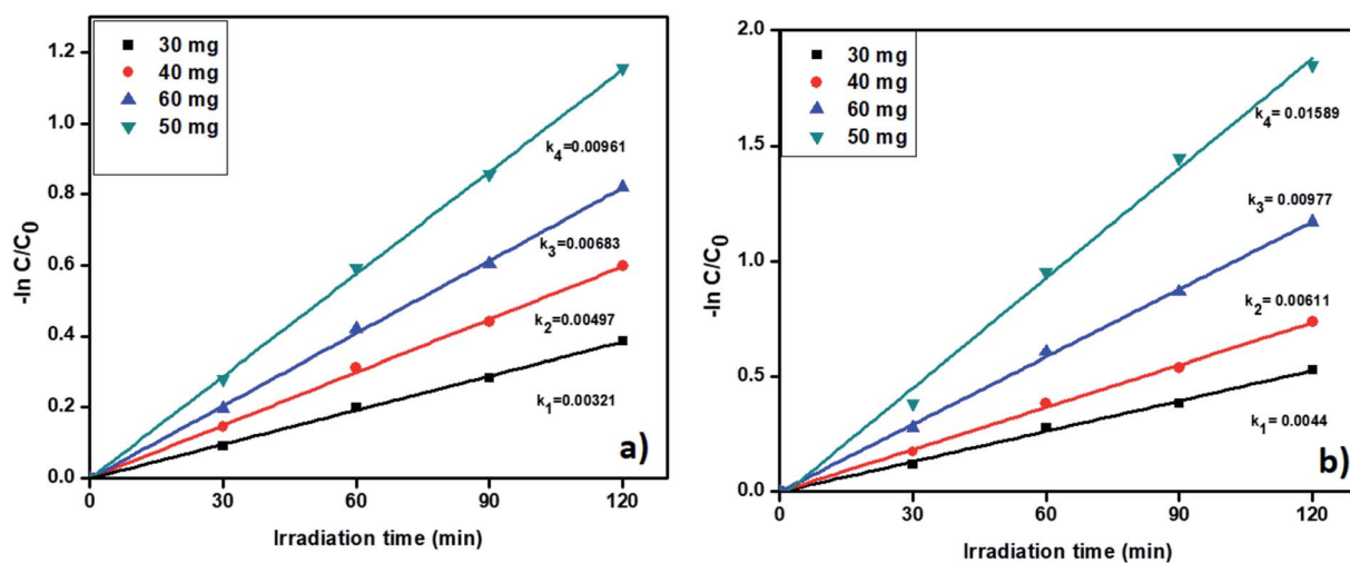
Fig. 10 The kinetic data for effect of catalyst on (a) TC oxidation and (b) Cr(vi) reduction (2 h of irradiation time, 20 ppm of TC, 20 ppm of Cr(vi), pH = 5 of TC, pH = 4 of Cr(vi)).
