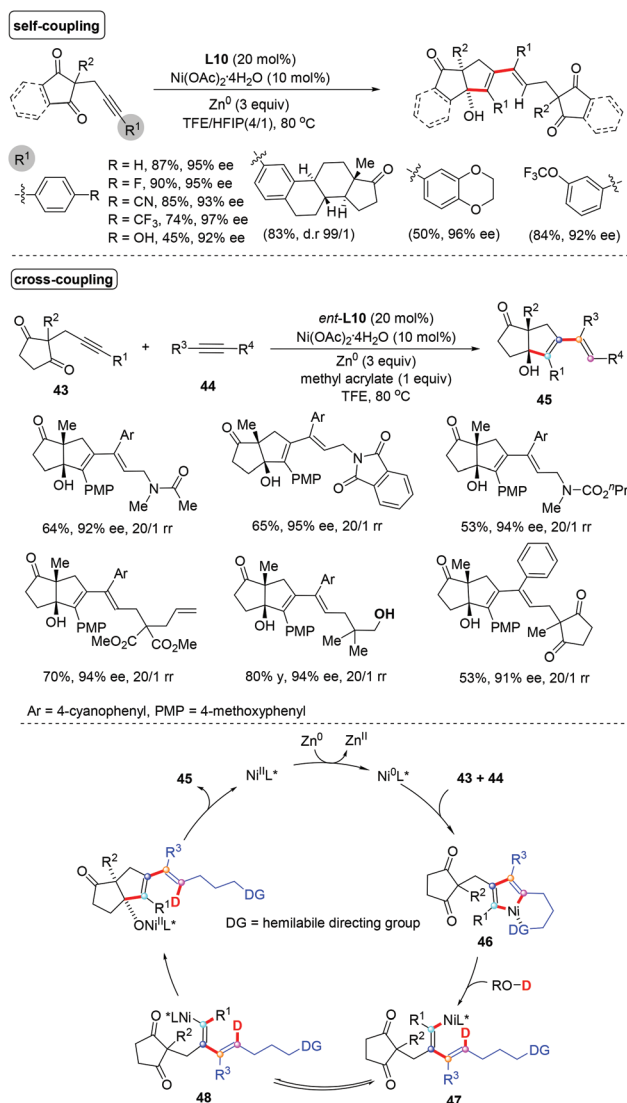
Scheme 32 Ni-Catalyzed reductive coupling of unsymmetrical internal alkynes.
