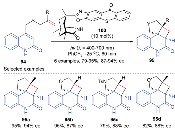
Scheme 28 Chiral thioxanthalone catalyzed [2 + 2] photocycloaddition reactions of 4-tethered quinolones.
