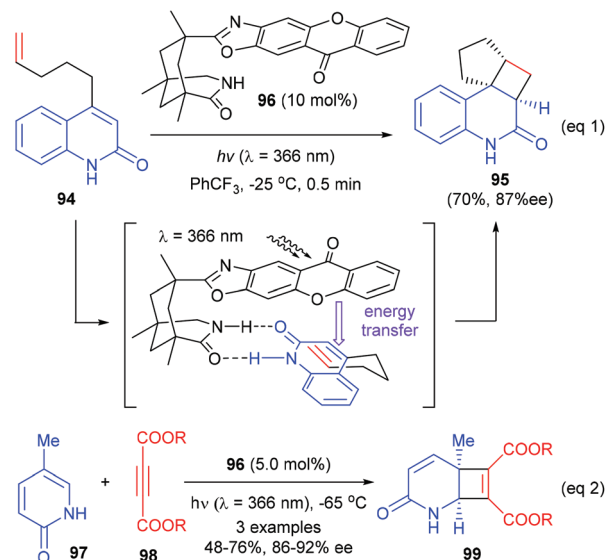
Scheme 27 [2 + 2]-Photocycloaddition reactions catalyzed by xanthalone-based organocatalyst.
