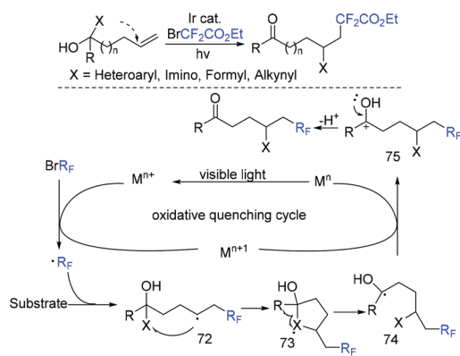
Scheme 41 The synthesis of difluorinated alkyl ketones.
