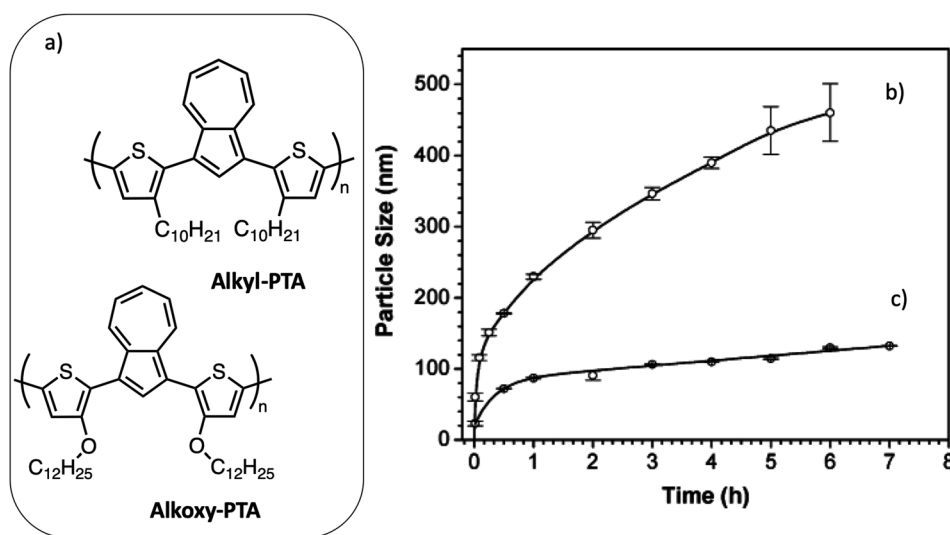
Fig. 9 (a) Chemical structures of poly(1,3-bis[2-(3- n -decylthienyl)]azulene) ( C_{10}H_{21} -PTA) and poly(1,3-bis[2-(3- n -dodecoxythienyl)]azulene) ( C_{12}H_{25}O -PTA). Time-dependent size evolutions of conjugated polymer nanoparticles in 1 : 1 mixed chloroform/methanol solutions containing (b) 10^{-5} M C_{10}H_{21} -PTA and (c) 10^{-5} M C_{12}H_{25}O -PTA. Adapted with permission from ref. 40 (Copyright 2005 Wiley-VCH Verlag).
