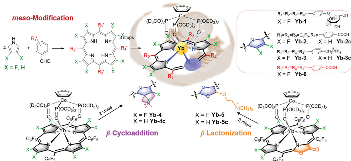
Fig. 8 Synthesis of biocompatible β-fluorinated Yb 3+ complexes.
