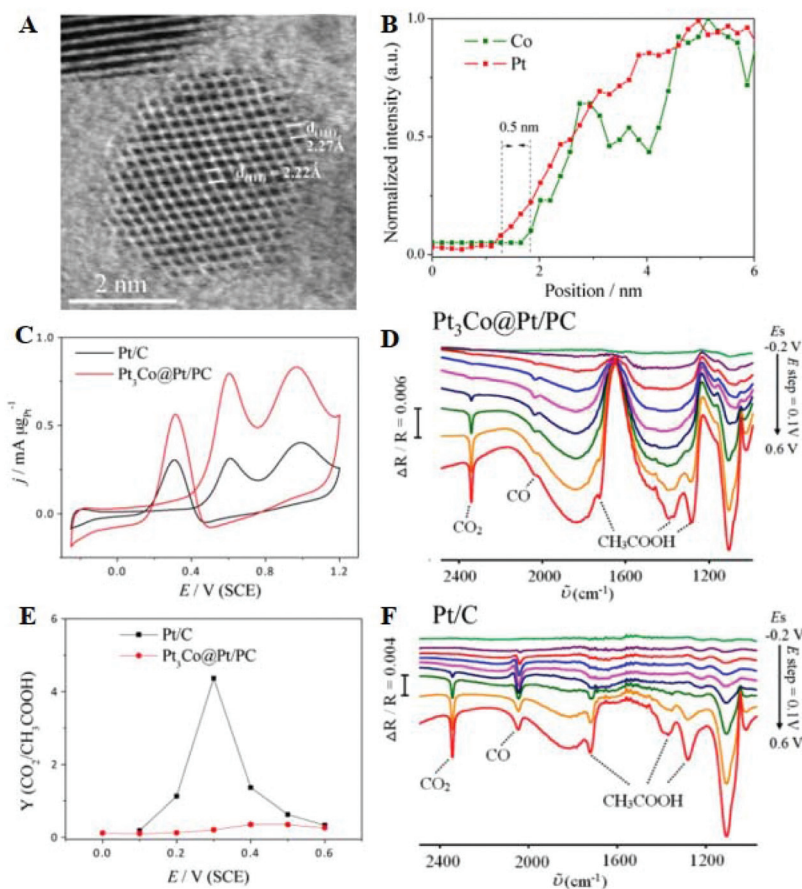
Fig. 6 (A) Atomic-resolution ADF-STEM image and (B) line-profile analysis of \text{Pt}_3\text{Co}@/\text{Pt}/\text{PC} nanoparticles. (C) CVs in 0.1 M \text{CH}_3\text{CH}_2\text{OH} + 0.1 M \text{HClO}_4 solution. (D) and (F) In situ FTIRS of \text{Pt}_3\text{Co}@/\text{Pt}/\text{PC} and \text{Pt}/\text{C} in 0.1 M \text{CH}_3\text{CH}_2\text{OH} + 0.1 M \text{HClO}_4 . (E) Ratio of integrated intensities of \text{CO}_2 and intensities of \text{CH}_3\text{COOH} as a function of working potential. Reproduced with permission from ref. 117. Copyright 2016, American Chemical Society.
