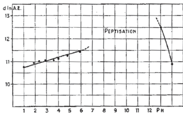
Fig. 2 Inter-layer distance value provided by d(001) from XRD experiments as a function of pH. 85 Graphite oxide spontaneously disperses into graphene oxide for the interval of pH marked as “peptisation”.
