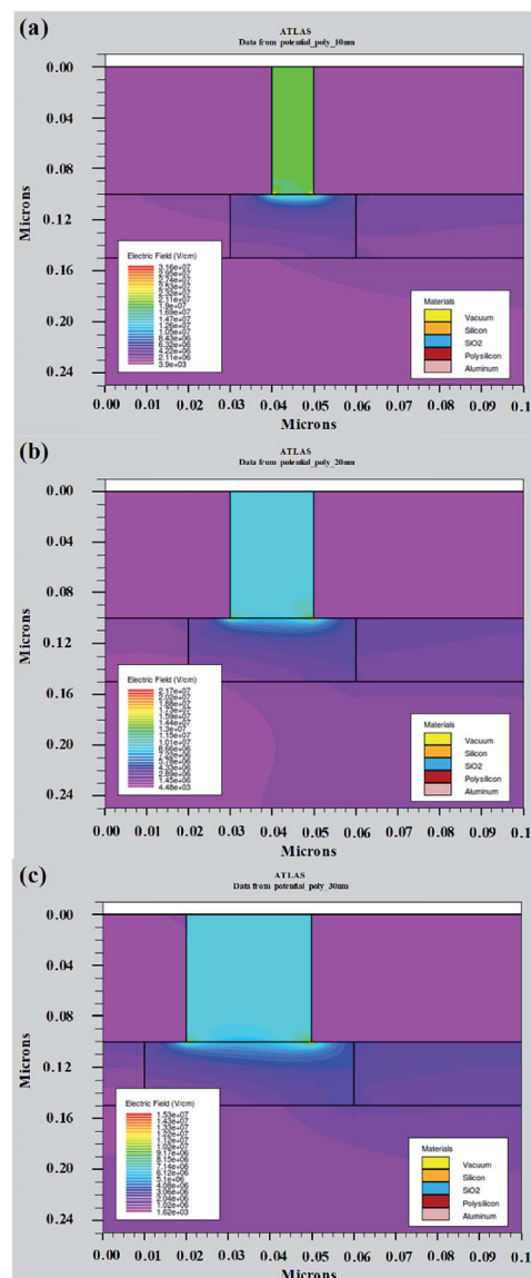
Fig. 2 The electric field intensity distribution of nanoscale vacuum channels with various lengths, (a) 10 nm, (b) 20 nm and (c) 30 nm.
