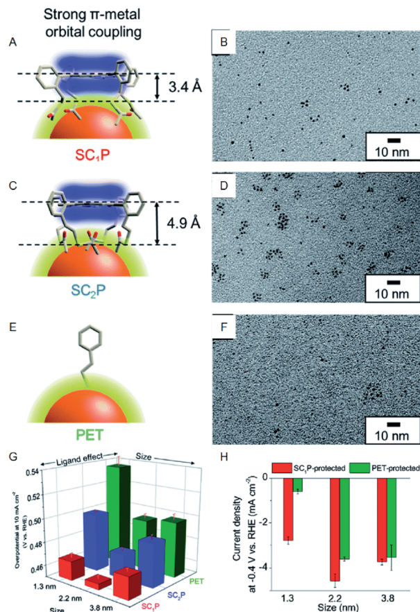
Fig. 3 (A), (C), and (E) Schematic of coordination fashions of \text{SC}_{1\text{P}} . (A) Tetrakis-5 \alpha ,10 \alpha ,15 \alpha ,20 \alpha -(2-acetylthioethylphenyl) porphyrin ( \text{SC}_{2\text{P}} ; A) and PET (E) at the surface of Au NCs. (B), (D), and (F) TEM images of 1.3, 2.2, and 3.8 nm Au NCs protected with \text{SC}_{1\text{P}} , respectively. (G) Comparison of overpotential at -10 \text{ mA cm}^{-2} . (H) Current density at -0.4 V of each size of Au NCs protected with each ligand. Panels (a)–(h) are reproduced with permission from ref. 27. Copyright 2018 Royal Society of Chemistry.
