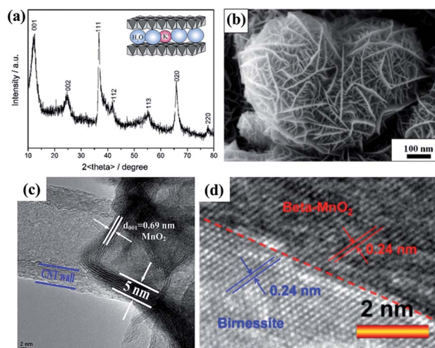
Fig. 2 (a) Typical XRD pattern of birnessite. 65 (b) SEM image of typical birnessite. 67 (c) and (d) HRTEM images of typical birnessite. 49,68
