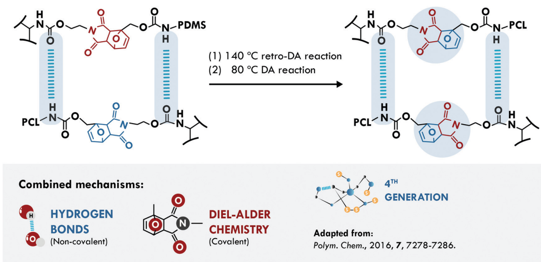
Fig. 11 Combination between DA chemistry and hydrogen bonds in PDMS-DA-PU. 200 ©2016. Adapted with permission from the Royal Society of Chemistry.
