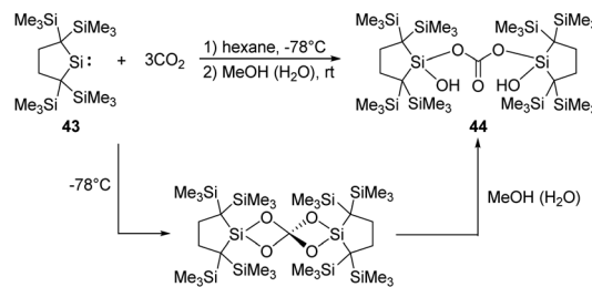
Scheme 20 Synthesis of the bis(silyl)carbonate 44 by the reaction of dialkylsilylene 43 with CO 2 .
