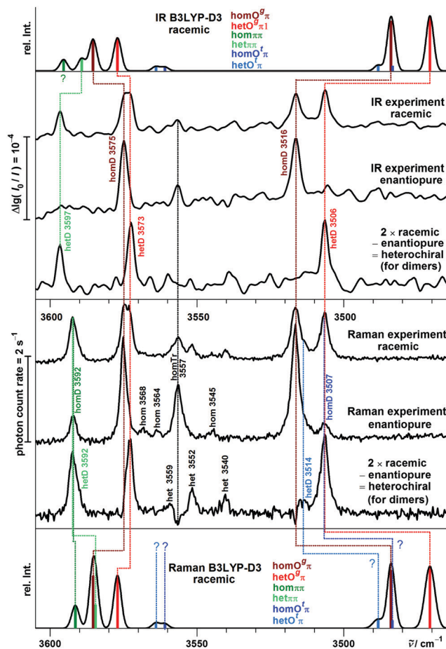
Fig. 10 P dimer B3LYP-D3 simulations (outer, racemic only, separate equilibria for hom and het) compared to experimental IR and Raman jet spectra (inner traces) after shifting the harmonic OH stretching wavenumbers by -165.2\text{ cm}^{-1} to match the monomer transition. A uniform conformational temperature of 100\text{ K} and a Gaussian FWHM of 3\text{ cm}^{-1} are assumed.
