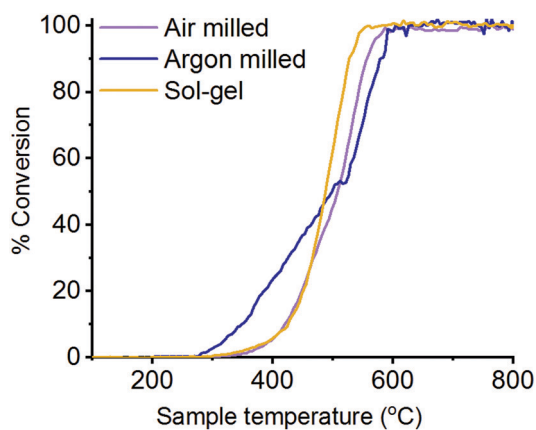
Fig. 10 Light-off curve of the percentage of \text{deN}_2\text{O} to \text{N}_2 over \text{LaMnO}_3 catalysts synthesised by mechanochemistry and sol-gel synthesised with 0.5% \text{N}_2\text{O}/\text{He} at 30 mL \text{min}^{-1} with a pre-treatment of He at 30 mL \text{min}^{-1} .
