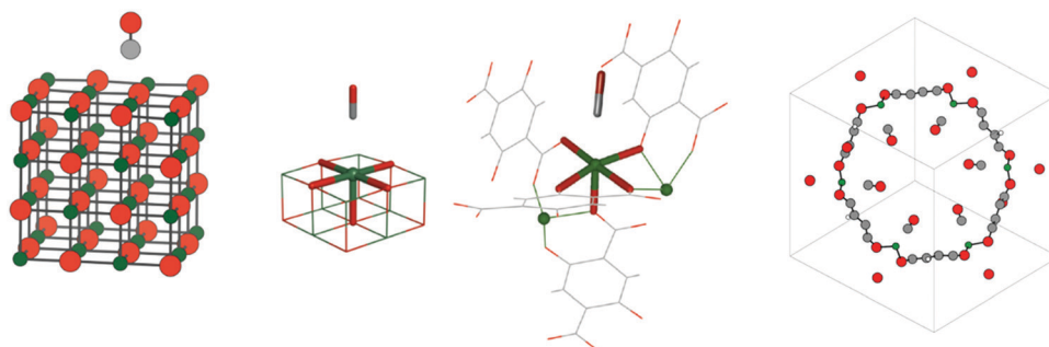
Fig. 1 Left: CO on a 4 layer MgO slab with a 4 \times 4 surface cell. Center: Five-fold coordinated Mg 2+ surface ions on the MgO(001) surface (center left) and in Mg 2 (dobdc) (center right). Right: Unit cell for CO in Mg 2 (dobdc). Color code: Mg – green, O – red, C – grey, H – white.
