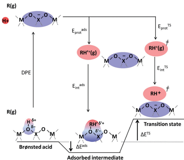
Scheme 2 A thermochemical cycle accounting for the thermodynamic properties of reactive intermediates ( \Delta E^{ads} ) and transition states ( \Delta E^{TS} ) involved in acid catalysis in terms of the DPE of the acid, the energies to form gaseous analogs of reactive intermediates and transition states from a free proton ( E_{prot}^{ads} , E_{prot}^{TS} ), and the energies of interaction of cations with the conjugate anion ( E_{int}^{ads} , E_{int}^{TS} ).
