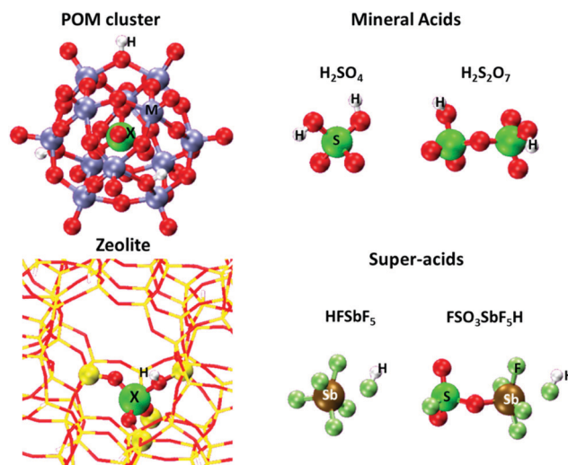
Fig. 1 Optimized structures of a H_3PMO_{12}O_{40} POM cluster, a cluster representation of Al-MFI heterosilicate, and molecular Brønsted acids. The acid composition in POM and MFI is modified by changing the heteroatom (X) in POM and MFI and addenda atoms (M) in POM clusters. Adapted from data and methods reported in ref. 30, 41 and 42.
