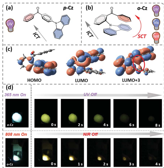
Fig. 1 (a) Chemical structure of p -Cz, the grey arrow represents through-bond intramolecular charge transfer (ICT); (b) chemical structure of o -Cz, the red arrow represents space charge transfer (SCT); (c) molecular orbital amplitude plots of HOMO, LUMO, and LUMO+3 of o -Cz, the red circle indicates the spatial orbital overlap of the donor and acceptor units; (d) photographs of o -Cz under UV-light and NIR-light irradiation and after the excitation source is turned off.
