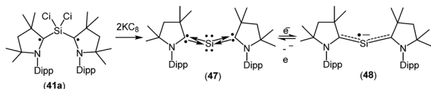
Fig. 13 cAAC-stabilized siladibene and in situ generation of (^{\text{Me}^2\text{cAAC}}_2\text{Si})^{\bullet-} .
