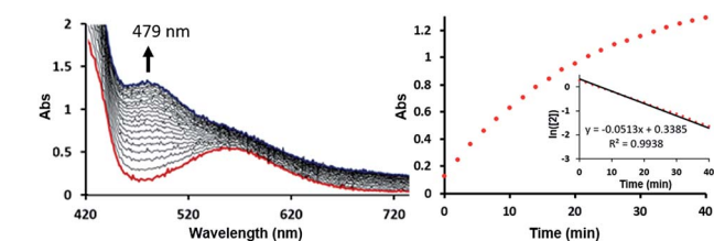
Fig. 7 Time stacked absorption spectra indicating consumption of 2 and formation of 3 with time (left). Plot of absorption at 479 nm vs. time (right); inset: plot of \ln[2] vs. time with linear least-squares fit.
