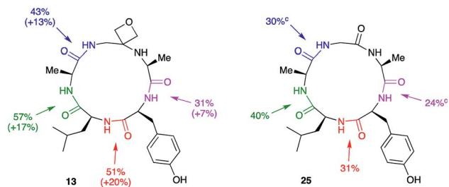
Fig. 5 Macrocyclisation efficiency as a function of location of oxetane relative to forming amide bond. a,b Reaction conditions: DEPBT (2 equiv.), 1 Pr 2 EtN (2 equiv.), DMF (0.001 M), RT, 24 h. c Taken from ref. 12.
