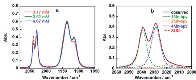
Fig. 5 IR spectra of fac -[Mn(bpy)(CO) 3 (MeCN)] + in DMF containing 1.3 M TEOA and different concentrations of CO 2 (a) and the curve-fitting result for the observed spectra at 3.17 mM CO 2 (b).
