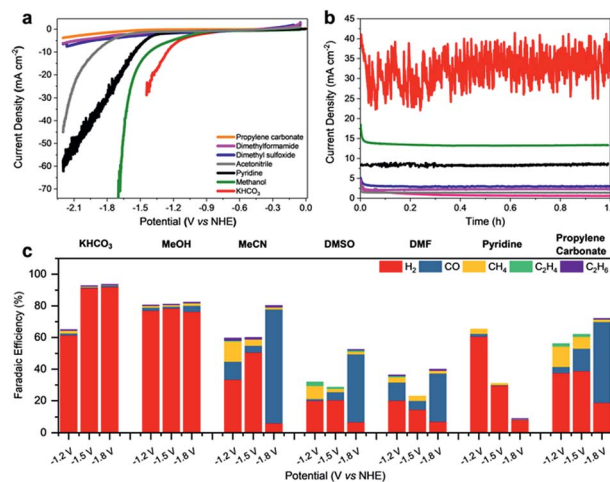
Fig. 2 (a) Linear sweep voltammograms recorded at 5 \text{ mV s}^{-1} in saturated \text{CO}_2 solutions. (b) Controlled potential coulometry (CPC) was performed in different electrolytes ( 0.1 \text{ M TBAPF}_6 ) at -1.80 \text{ V vs. NHE} and (c) the composition of the \text{CO}_2 reduction products analyzed by on-line gas chromatography after 1 h. Notably, formation of soluble reduction products was not observed in additionally performed GC and HPLC experiments.
