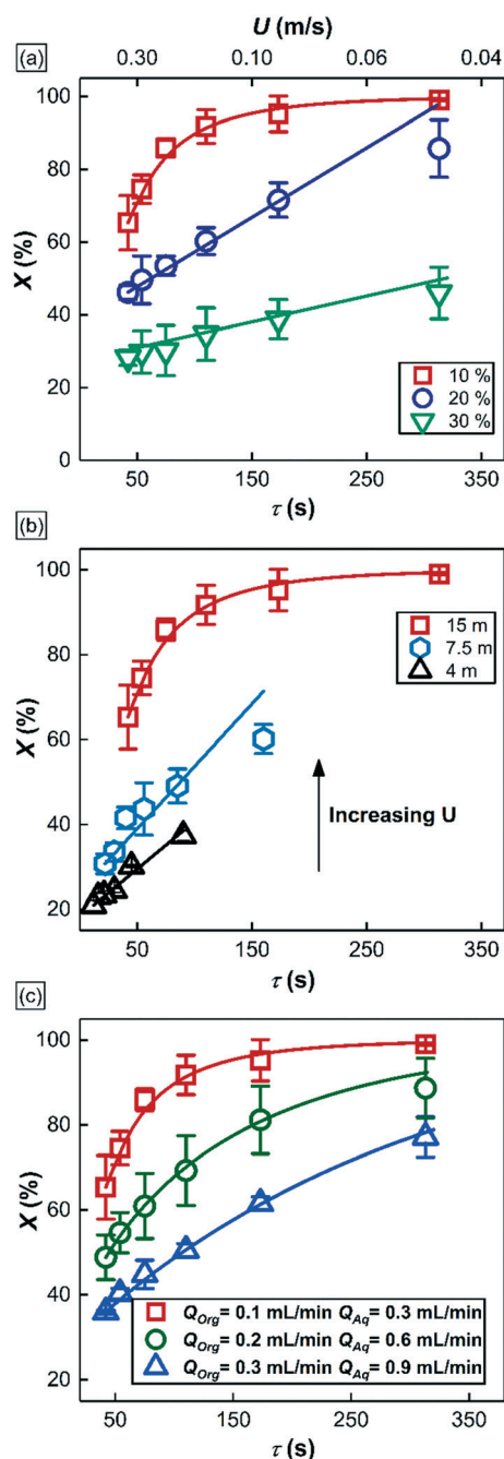
Fig. 6 1-Hexene conversion ( X ) versus bubble residence time ( \tau = L_R/U ) at various operational conditions. 1-Hexene conversion was calculated as X = (C_{hex,0} - C_{hex})/C_{hex,0} where, C_{hex,0} is the initial 1-hexene concentration and C_{hex} is the concentration of 1-hexene in the reactor effluent at different bubble residence times, respectively. (a) The effect of starting 1-hexene concentration. C_{hex,0} = 0.8 M (10% v/v), 1.6 M (20% v/v), and 2.4 M (30% v/v). Q_{Org} = 0.1 mL min -1 , Q_{Aq} = 0.3 mL min -1 , L_R = 15 m. (b) The effect of the reactor length. C_{hex,0} = 0.8 M (10% v/v), Q_{Org} = 0.1 mL min -1 , Q_{Aq} = 0.3 mL min -1 . (c) The effect of total liquid flow rate Q_T at constant Q_{Org}:Q_{Aq} ratio of 1:3. C_{hex,0} = 0.8 M (10% v/v). Red: Q_{Org} = 0.1 mL min -1 , Q_{Aq} = 0.3 mL min -1 , green: Q_{Org} = 0.2 mL min -1 , Q_{Aq} = 0.6 mL min -1 , blue: Q_{Org} = 0.3 mL min -1 , Q_{Aq} = 0.9 mL min -1 and L_R = 15 m. Q_{Gas} = 12 –80 mL min -1 . C_{RhNP} = 1 mM for all different experimental conditions. Solid lines represent model predictions (section 3.3).
