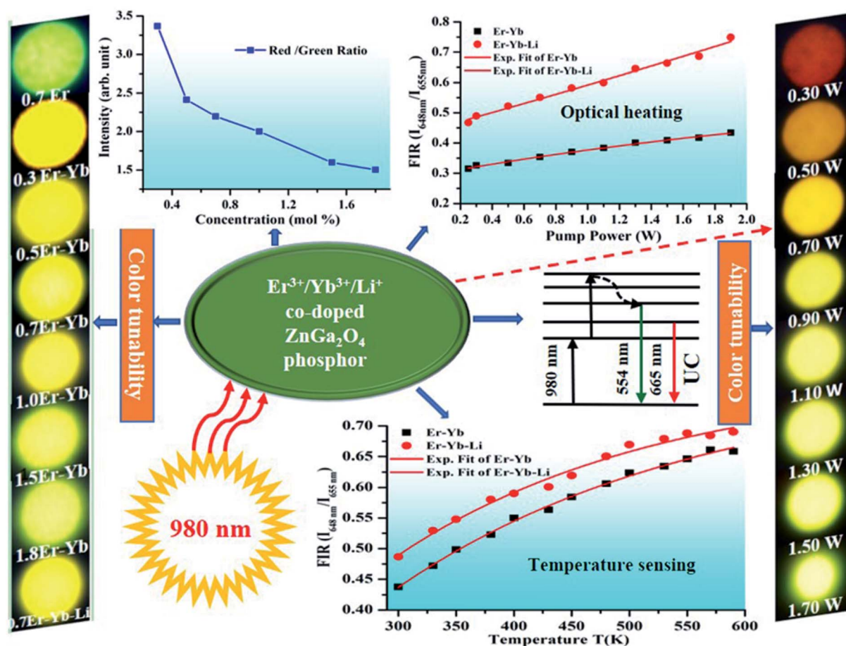
Fig. 18 Schematic model for color tunability, R/G ratio, energy level diagram, optical heating, and temperature sensing of the Er 3+ /Yb 3+ /Li + co-doped ZnGa 2 O 4 phosphor.
