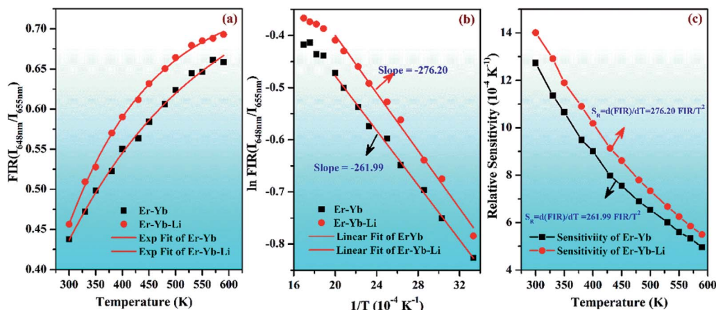
Fig. 17 (a) Plots of FIR ( I_{648\text{nm}}/I_{655\text{nm}} ) versus temperature, (b) \ln \text{FIR} (I_{648\text{nm}}/I_{655\text{nm}}) versus T^{-1} , and (c) sensitivity versus temperature for the 0.7\text{Er}^{3+}/\text{Yb}^{3+} and 0.7\text{Er}^{3+}/\text{Yb}^{3+}/\text{Li}^{+} co-doped \text{ZnGa}_2\text{O}_4 phosphors on excitation with 980 nm at 1 W.
