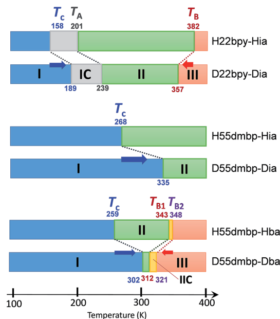
Fig. 6 Phase-transition sequences of H22bpy-Hia, H55dmbp-Hba, and their deuterated salts. The numbers represent the phase-transition temperatures in Kelvin.
