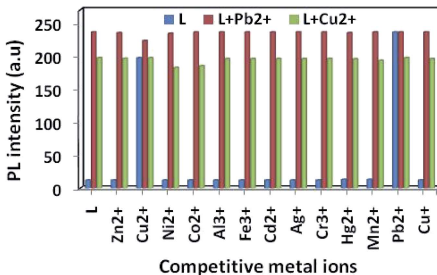
Fig. 6 Fluorescence intensity of L , (10 \mu\text{M} ) to 5 equiv. of \text{Cu}^{2+} , \text{Pb}^{2+} and other cations in \text{CH}_3\text{OH} –tris buffer ( 1 : 1 , v/v) mixture. Excited wave length 340 nm and emission maxima 412 nm for \text{Cu}^{2+} and 440 nm for \text{Pb}^{2+} .
