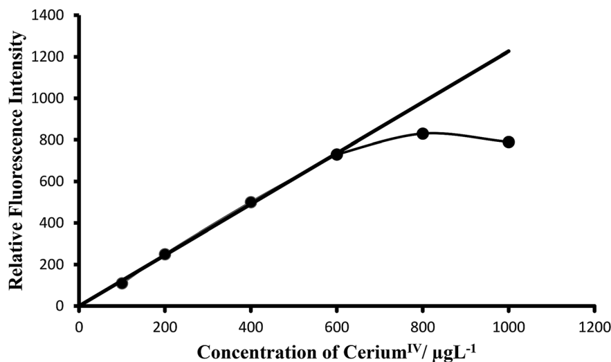
Fig. 7 Calibration graph F: 100–600 \mu\text{g L}^{-1} of cerium IV . Bandwidth: Ex. slit-1.5, Em. slit-1.5. Sensitivity: high.
