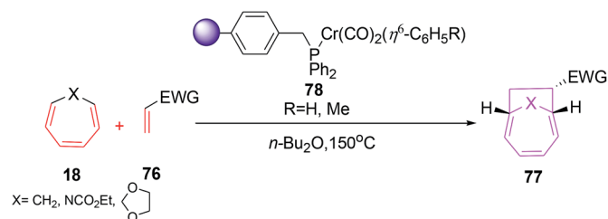
Scheme 30 [6 + 2] cycloadditions of CHT with ethyl acrylate catalysed by solid supported chromium(0) complex.
