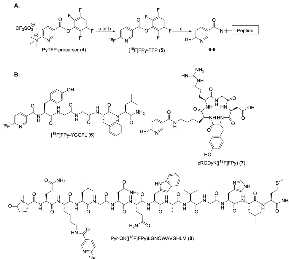
Scheme 1 (A) Radiolabeling of peptides with [18F]FPy-TFP (5). (B) Structures of radiolabeled [18F]FPy-peptides (6–8). Reagents and conditions: (a) [18F]F, K 2 222, K 2 CO 3 , 4 : 1 tBuOH : MeCN, 40 °C, 10 min or (b) [18F]F, TBA-HCO 3 , 4 : 1 tBuOH : MeCN, 40 °C, 10 min. (c) Peptide (1 mg), DMSO, DIPEA, 40 °C, 15 min.
