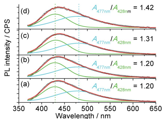
Fig. 5 Representative PL spectra of the pristine carbon dots (a), with 100 \mu\text{M } Fe^{3+} (b), 88 \mu\text{M } H_2O_2 (c) and 100 \mu\text{M } Fe^{3+} plus 4.4 \mu\text{M } H_2O_2 (d). The excitation wavelength was 360 nm and A_{477 \text{ nm}}/A_{428 \text{ nm}} indicates the ratio of the area between the peaks at 477 nm and 428 nm. The R^2 value of the fitting of the curves was 0.996.
