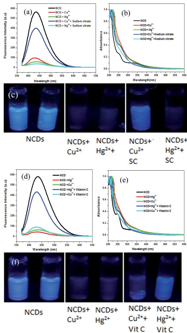
Fig. 5 (a) Fluorescence emission spectra of NCDs (2 mL) before and after addition of Hg 2+ , Cu 2+ ([M n+ ] = 50 \mu M, 10 \mu L) and then trisodium citrate (SC = 50 \mu M, 10 \mu L); (b) UV-visible spectrum of NCDs before and after addition of Hg 2+ , Cu 2+ , trisodium citrate ([M n+ ] and/or SC = 50 \mu M, 10 \mu L); (c) corresponding digital photograph under 365 nm UV light; (d) fluorescence emission spectra of NCDs (2 mL) before and after addition of Hg 2+ , Cu 2+ , vitamin C ([M n+ ] and/or Vit C = 50 \mu M, 10 \mu L); (e) UV-visible spectrum of NCDs before and after addition of Hg 2+ , Cu 2+ , vitamin C ([M n+ ] and/or Vit C = 50 \mu M, 10 \mu L); (f) corresponding digital photograph under 365 nm UV light.
