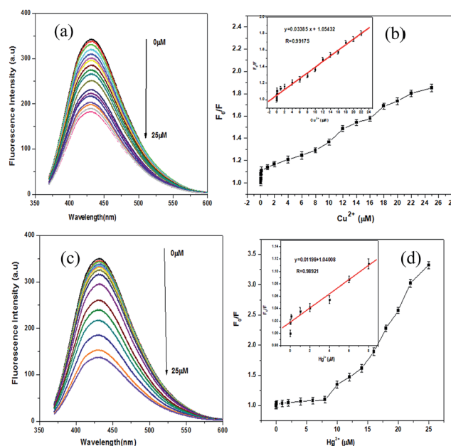
Fig. 6 (a) Fluorescence emission responses of aqueous NCDs on addition of Cu 2+ (0–25 \mu M) ions with excitation wavelength fixed at 360 nm; (b) plot of F_0/F vs. Cu 2+ concentration (0–25 \mu M), error bars are derived from three independent sets of experiments. (c) Fluorescence emission responses of aqueous NCDs on addition of Hg 2+ (0–25 \mu M) ions with excitation wavelength fixed at 360 nm; (d) plot of F_0/F vs. Hg 2+ concentration (0–25 \mu M), error bars are derived from three independent sets of experiments.
