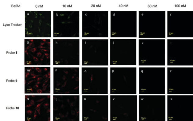
Fig. 12 Lysosomal pH dependent staining of A549 cells with probe 8 (10 \mu M), probe 9 (10 \mu M), probe 10 (10 \mu M) and LysoTracker green DND-26 (0.5 \mu M). A549 cells pretreated with or without Bafilomycin A1 for about 5 h and then analyzed by confocal microscopy. The intracellular fluorescence of probes 9 and 10 is shown in red and that of LysoTracker green DND-26 is shown in green. Copyright 2015 Elsevier.
