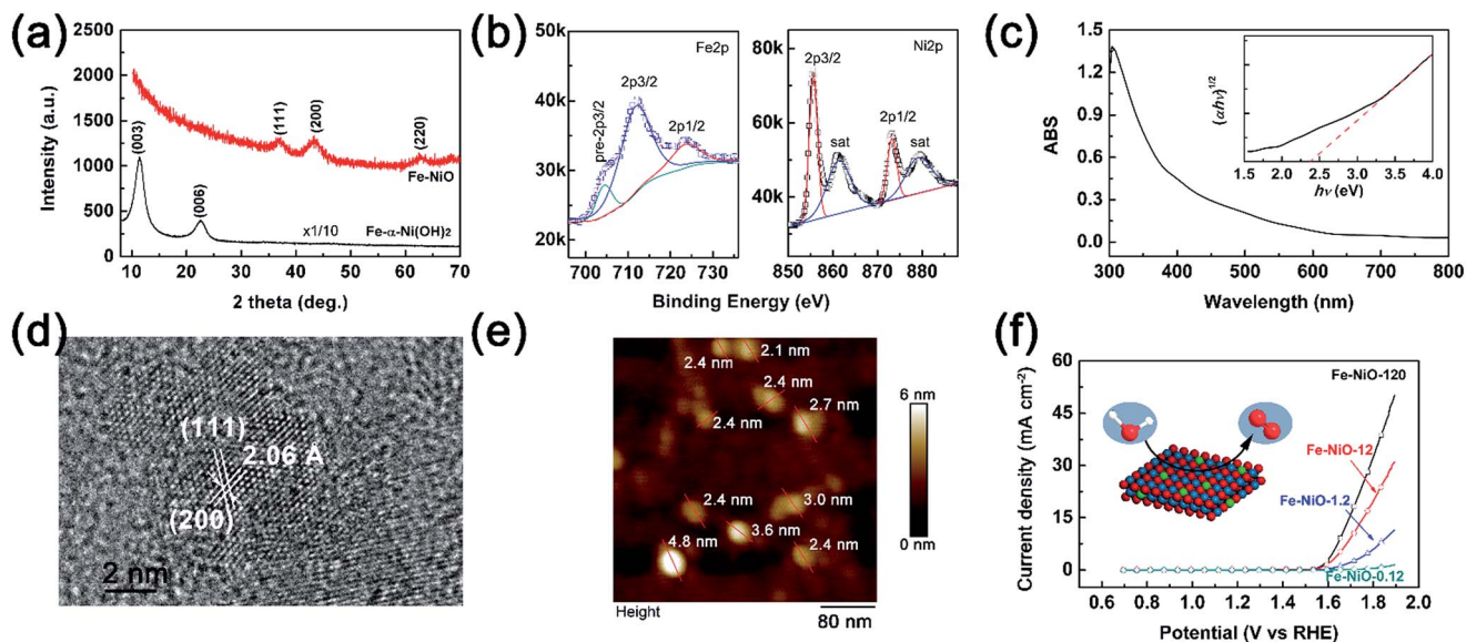
Fig. 1 (a) XRD patterns of the Fe-doped Ni(OH) 2 precipitate (black curve at bottom) and Fe-doped NiO (red curve on the top); (b) XPS spectra of the Fe-NiO film (left: Fe2p; right: Ni2p); (c) UV-vis absorption spectrum of the Fe-NiO film, the inset was the Tauc plot of indirect band estimation; (d) HR-TEM image of the Fe-NiO nanosheet; (e) AFM height image of the Fe-NiO nanosheets; (f) J - V curves of the Fe-NiO nanosheets on FTO prepared with various concentrations in a 1 M NaOH electrolyte, and a scanning rate of 20 mV s -1 .
