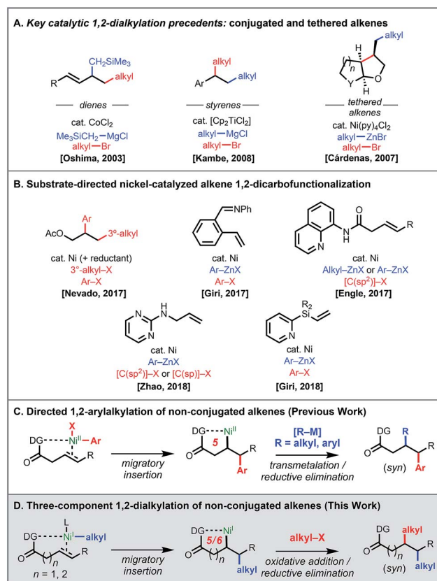
Scheme 1 Three-component 1,2-dicarbonylation with C(sp^3) reaction partners: precedents and current work.
