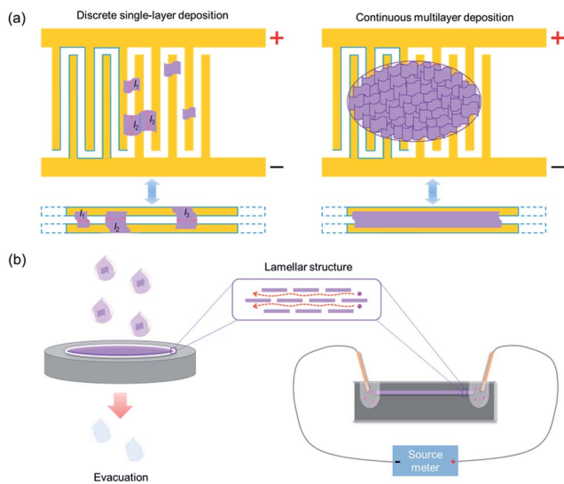
Fig. 2 Schematic diagrams for H^+/OH^- ion conductivity measurements in the case of 2D materials. (a) Comb-like microelectrode assisted measurement and (b) lamellar membrane assisted measurement.
