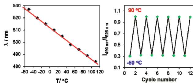
Fig. 7 Left: diagram showing the linear dependence of the emission \lambda_{\text{max}} of BO-1 fluorescence in MOE on T from 223 K ( -50\text{ }^\circ\text{C} ) to 383 K ( 110\text{ }^\circ\text{C} ). Right: diagram showing the reversible cycling of BO-1 emission between -50\text{ }^\circ\text{C} and 90\text{ }^\circ\text{C} , plotted with the intensity ratio of I_{490\text{ nm}}/I_{525\text{ nm}} vs. T .
